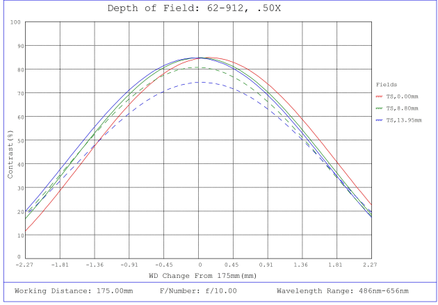
#62-912, 0.5X, 28.7mm F-Mount PlatinumTL™ Telecentric Lens, Depth of Field Plot, 175mm Working Distance, f10
