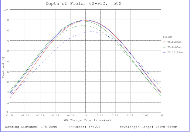
#62-912, 0.5X, 28.7mm F-Mount PlatinumTL™ Telecentric Lens, Depth of Field Plot, 175mm Working Distance, f6
