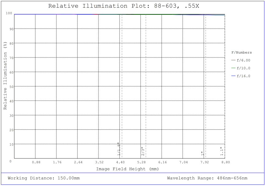
#88-603, 0.55X CobaltTL Telecentric Lens, Relative Illumination Plot
