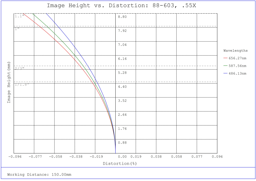
#88-603, 0.55X CobaltTL Telecentric Lens, Distortion Plot
