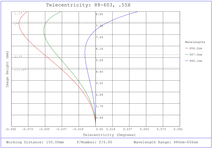
#88-603, 0.55X CobaltTL Telecentric Lens, Telecentricity Plot
