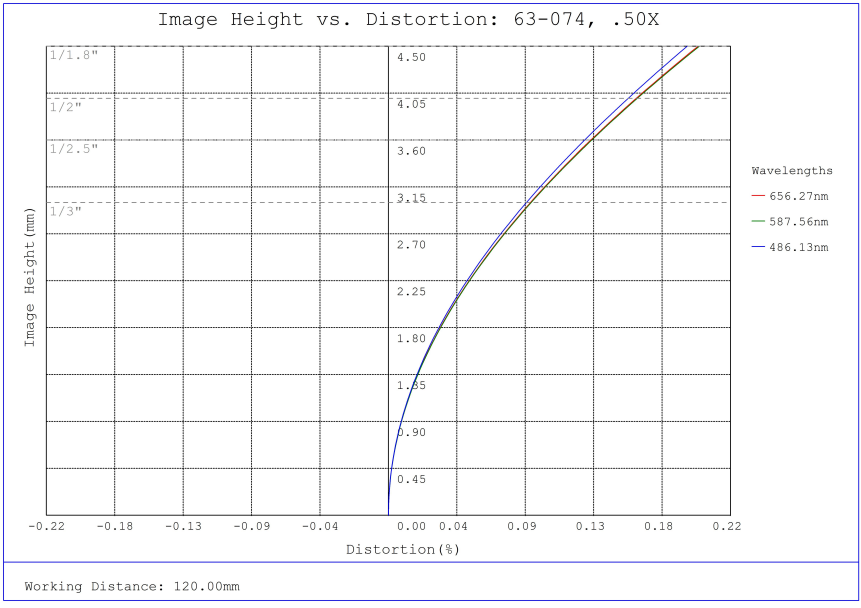
#63-074, 0.50X SilverTL™ Telecentric Lens, Distortion Plot
