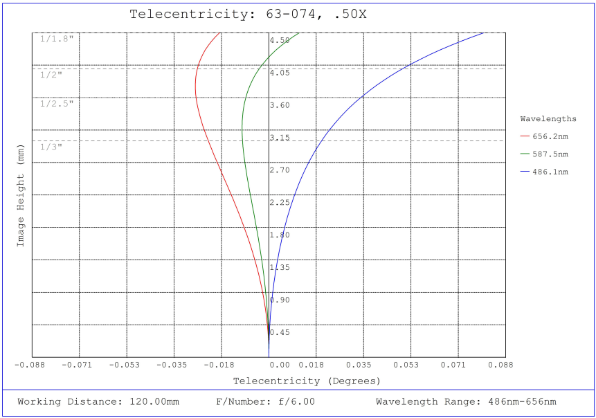
#63-074, 0.50X SilverTL™ Telecentric Lens, Telecentricity Plot
