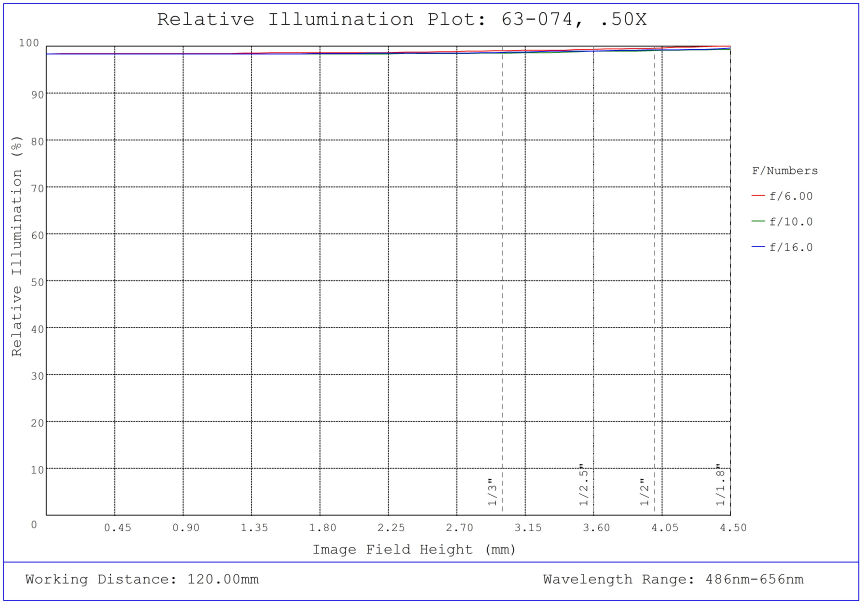
#63-074, 0.50X SilverTL™ Telecentric Lens, Relative Illumination Plot
