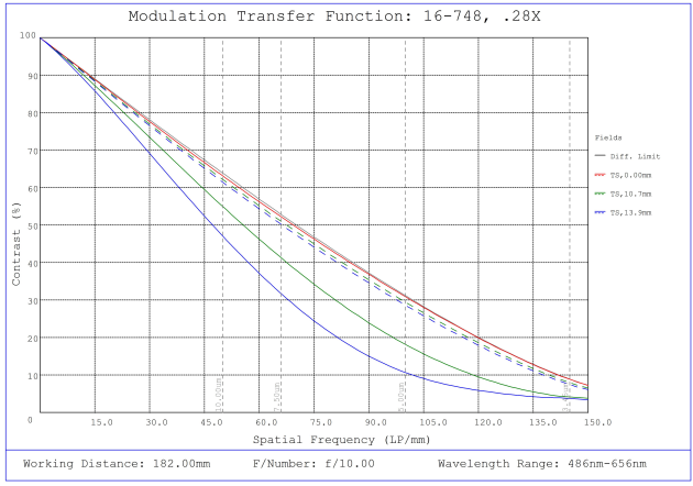
#16-748, 0.28X, 28.7mm TFL-Mount PlatinumTL™ Telecentric Lens, Modulated Transfer Function (MTF) Plot, 182mm Working Distance, f10
