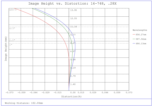
#16-748, 0.28X, 28.7mm TFL-Mount PlatinumTL™ Telecentric Lens, Distortion Plot
