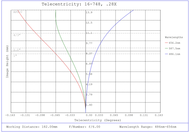
#16-748, 0.28X, 28.7mm TFL-Mount PlatinumTL™ Telecentric Lens, Telecentricity Plot
