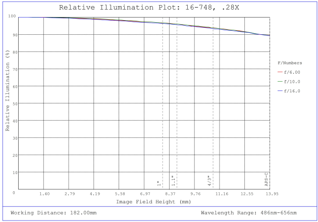
#16-748, 0.28X, 28.7mm TFL-Mount PlatinumTL™ Telecentric Lens, Relative Illumination Plot
