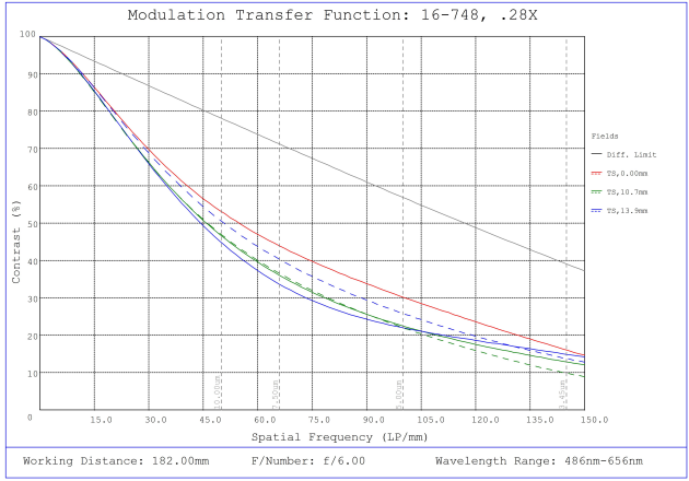
#16-748, 0.28X, 28.7mm TFL-Mount PlatinumTL™ Telecentric Lens, Modulated Transfer Function (MTF) Plot, 182mm Working Distance, f6
