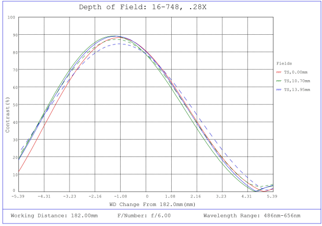
#16-748, 0.28X, 28.7mm TFL-Mount PlatinumTL™ Telecentric Lens, Depth of Field Plot, 182mm Working Distance, f6
