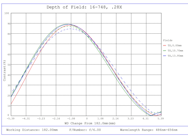
#16-748, 0.28X, 28.7mm TFL-Mount PlatinumTL™ Telecentric Lens, Depth of Field Plot, 182mm Working Distance, f6
