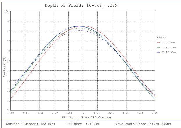
#16-748, 0.28X, 28.7mm TFL-Mount PlatinumTL™ Telecentric Lens, Depth of Field Plot, 182mm Working Distance, f10
