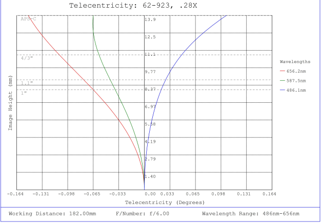
#62-923, 0.28X, 28.7mm M42 x 1.0 (6.56mm) PlatinumTL™ Telecentric Lens, Telecentricity Plot
