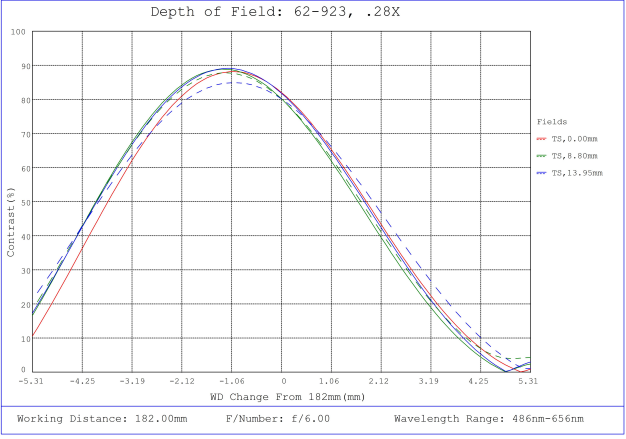
#62-923, 0.28X, 28.7mm M42 x 1.0 (6.56mm) PlatinumTL™ Telecentric Lens, Depth of Field Plot, 182mm Working Distance, f6
