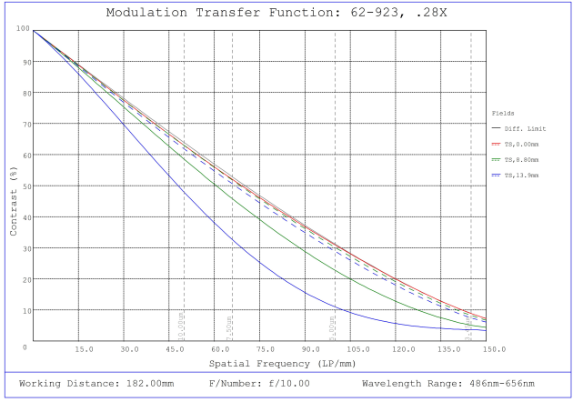
#62-923, 0.28X, 28.7mm M42 x 1.0 (6.56mm) PlatinumTL™ Telecentric Lens, Modulated Transfer Function (MTF) Plot, 182mm Working Distance, f10
