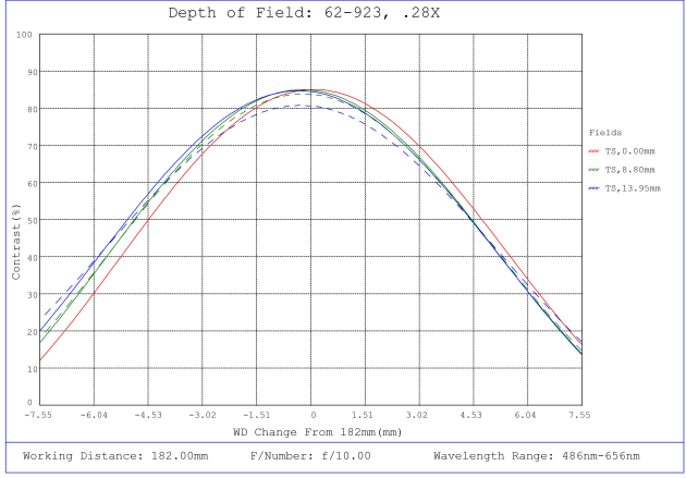
#62-923, 0.28X, 28.7mm M42 x 1.0 (6.56mm) PlatinumTL™ Telecentric Lens, Depth of Field Plot, 182mm Working Distance, f10
