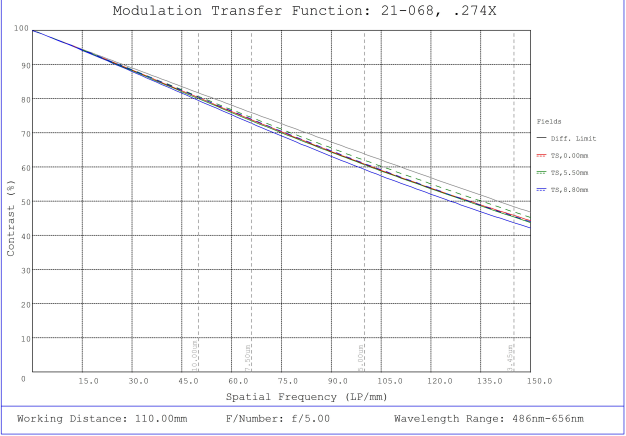
#21-068, 0.274X CobaltTL Telecentric Lens, Modulated Transfer Function (MTF) Plot, 110mm Working Distance, f5
