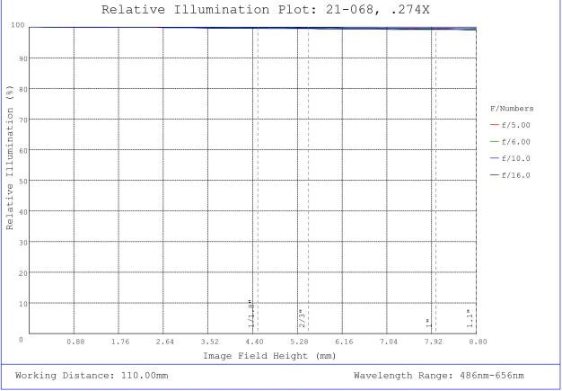
#21-068, 0.274X CobaltTL Telecentric Lens, Relative Illumination Plot
