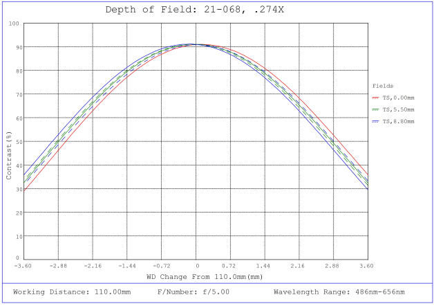
#21-068, 0.274X CobaltTL Telecentric Lens, Depth of Field Plot, 110mm Working Distance, f5
