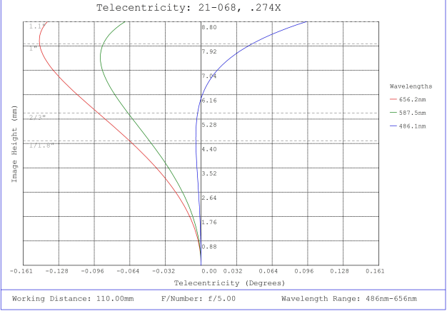
#21-068, 0.274X CobaltTL Telecentric Lens, Telecentricity Plot
