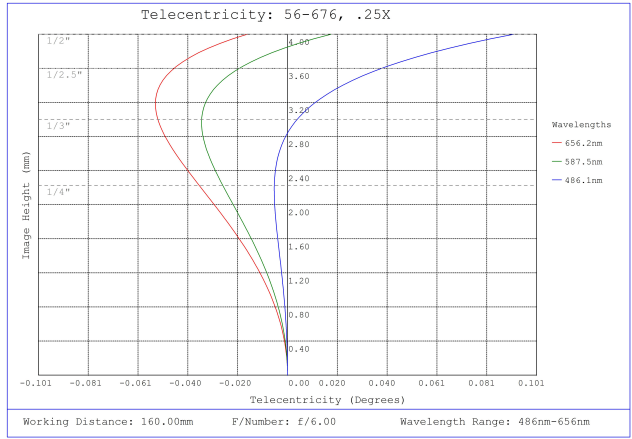
#56-676, 0.25X SilverTL™ Telecentric Lens, Telecentricity Plot
