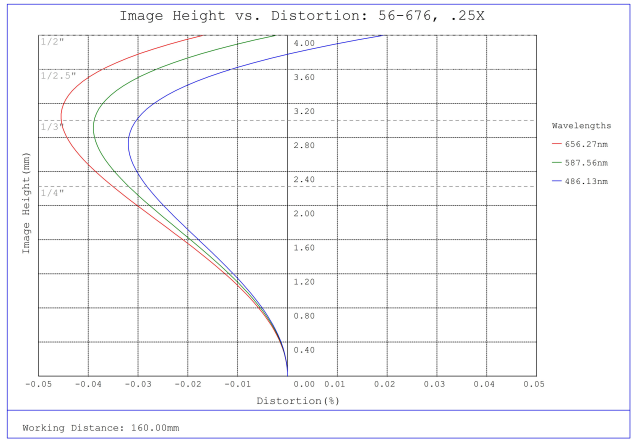
#56-676, 0.25X SilverTL™ Telecentric Lens, Distortion Plot
