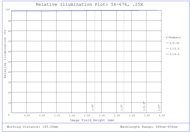
#56-676, 0.25X SilverTL™ Telecentric Lens, Relative Illumination Plot
