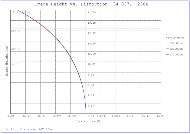
#34-037, 0.238X, 35mm M58 x 0.75 TitanTL® Telecentric Lens, Distortion Plot
