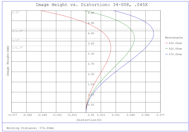
#34-008, 0.045X, 2/3" C-Mount TitanTL® Telecentric Lens, Distortion Plot
