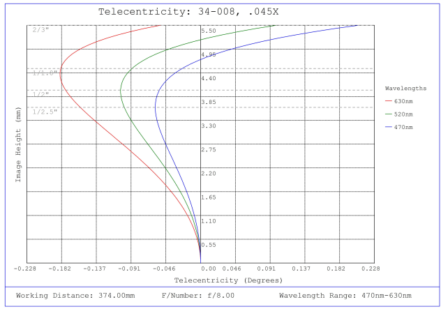
#34-008, 0.045X, 2/3" C-Mount TitanTL® Telecentric Lens, Telecentricity Plot
